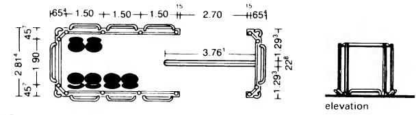
12 Waiting shelter on main line platforms, plan view
